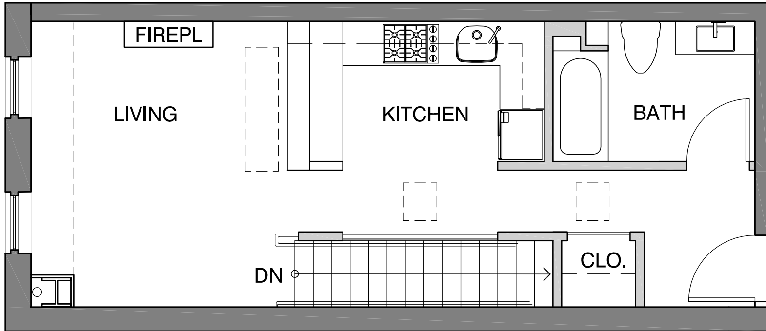
THIRD FLOOR
