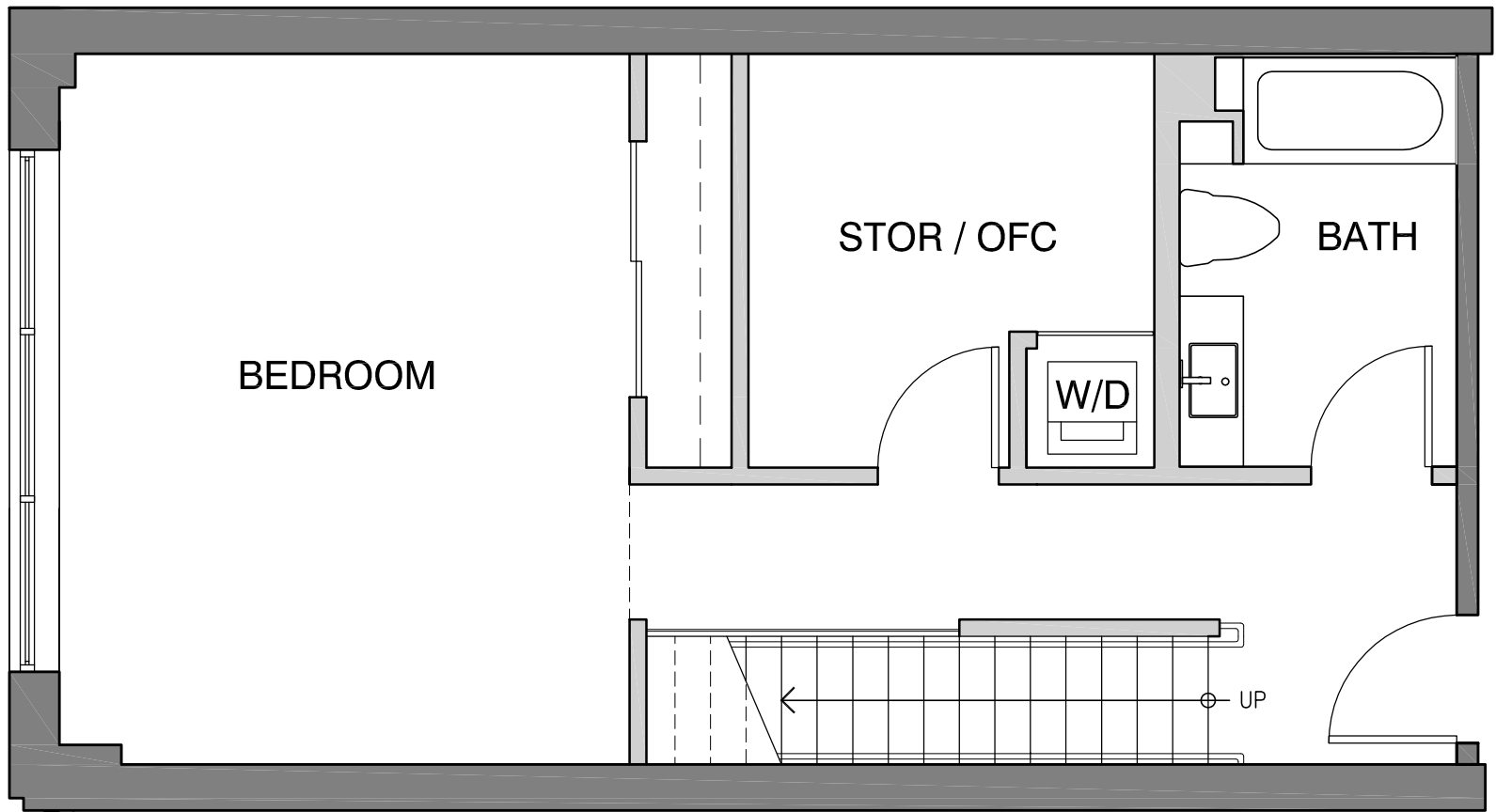
SECOND FLOOR
